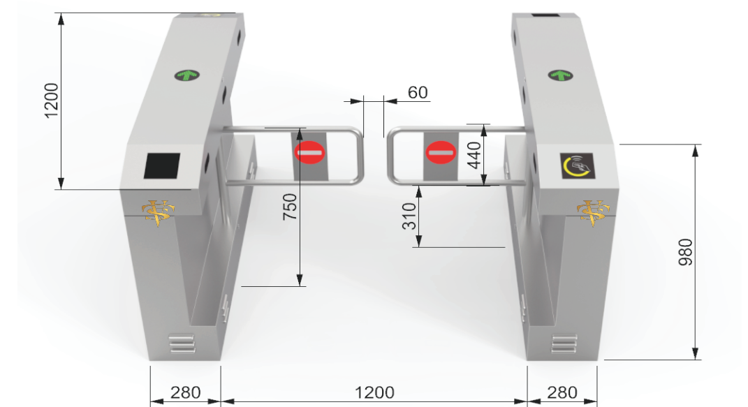
B904 (STANDARD STYLE PASSAGEWAY, MALL TRAILER CAN PASS)
