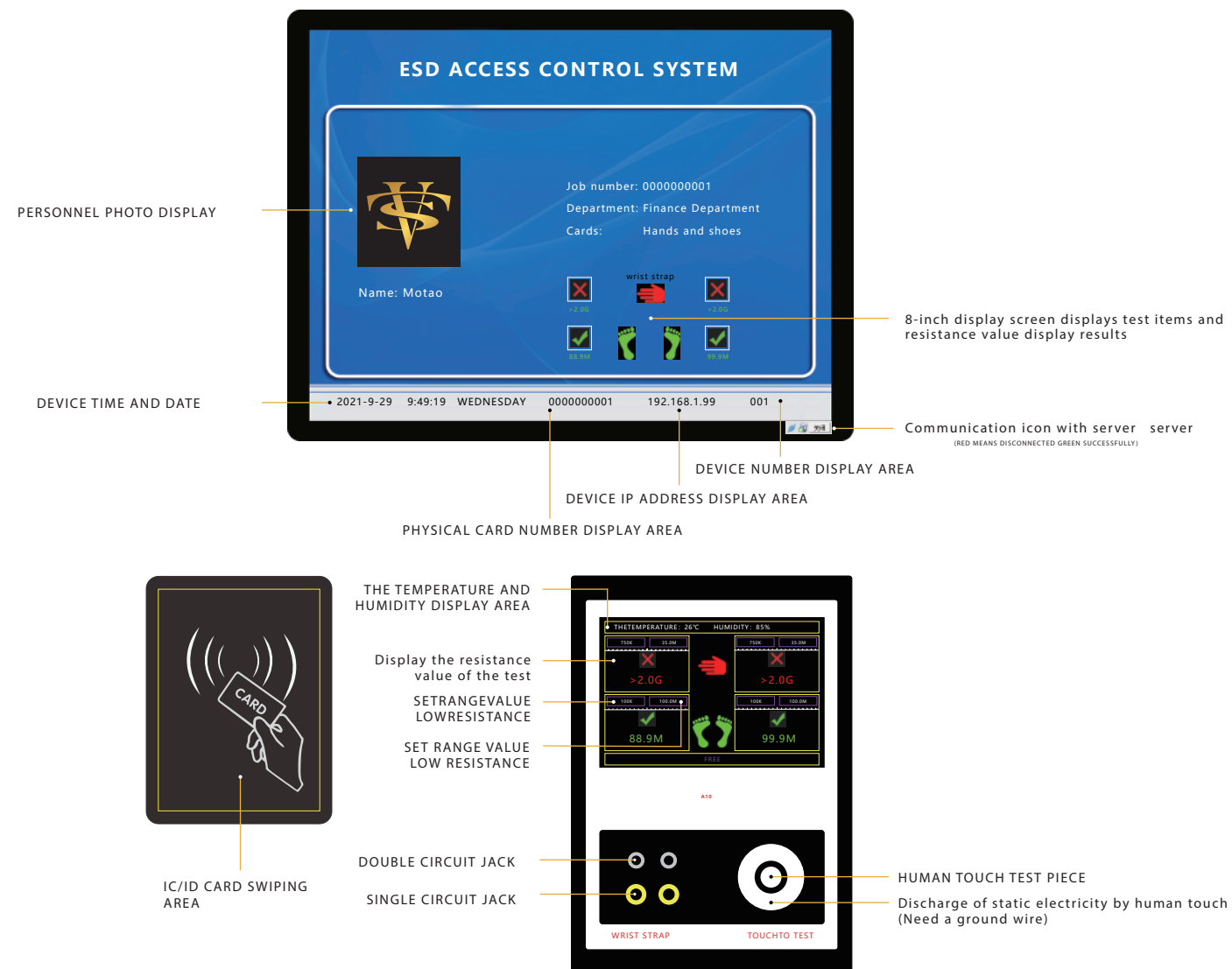
VT-T10 DIGITAL DISPLAY ESD TESTER
