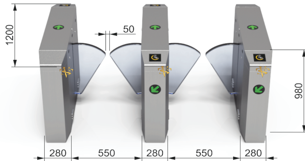
WING GATES (STANDARD STYLE PASSAGEWAY)
